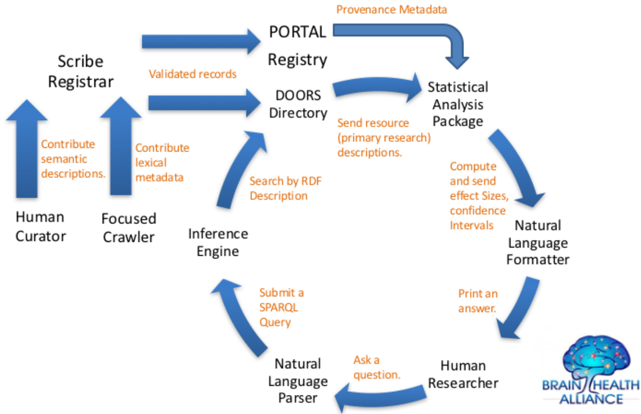
Figure 2: Flow of information between components in the proposed system for automated meta-analysis
